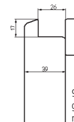
Facet profiel tbv glaspakket 26 mm
